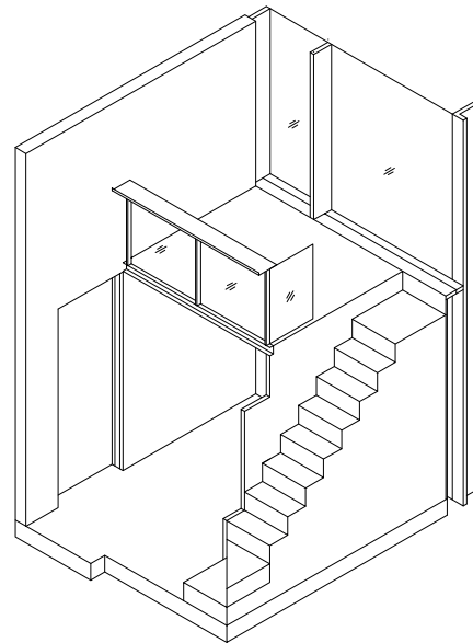
ISOMETRIC VIEW
